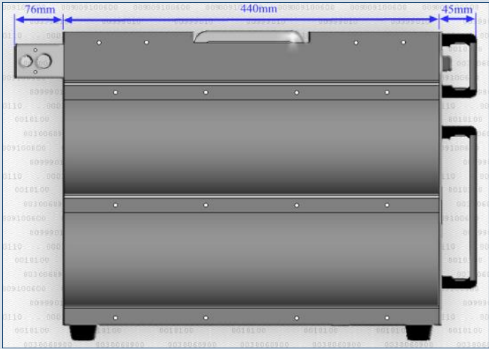
NL device with FK25 connections
