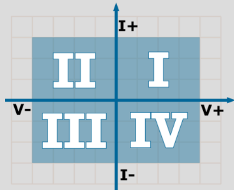
4-quadrant mode
